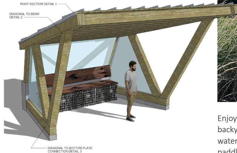
Rendering of causeway shelter design
